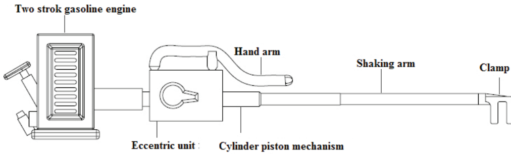
Figure 2- Eccentric type shaker used in experiments
