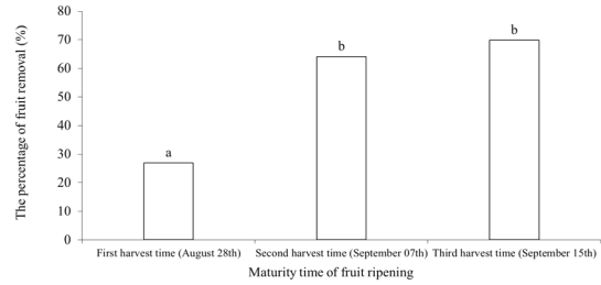
Figure 4- The percentages of fruit removal by eccentric type shaker in hazelnut harvesting subjected to maturity time of fruit ripening. Means in the same bar not sharing a common letter are significantly different ( P < 0.05 )
