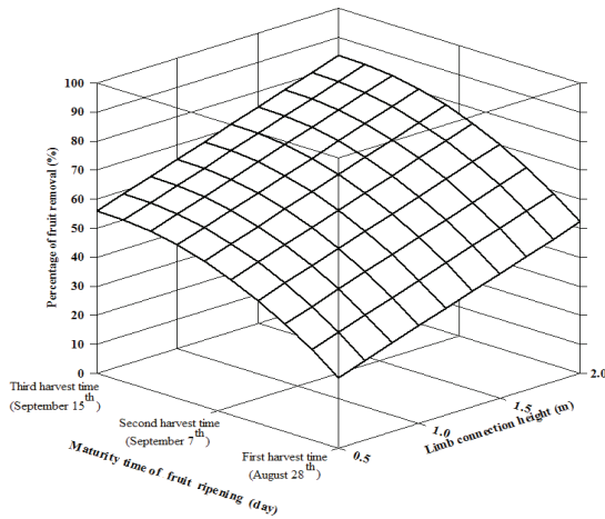
Figure 5- Changes in the percentage of fruit removal due to different limb connection heights and maturity time of fruit ripening in Yomra hazelnut cultivar
