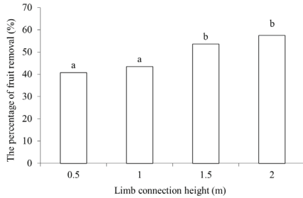
Figure 3- The percentages of fruit removal by eccentric type shaker in hazelnut harvesting subjected to different limb connection heights. Means in the same bar not sharing a common letter are significantly different ( P < 0.01 )
