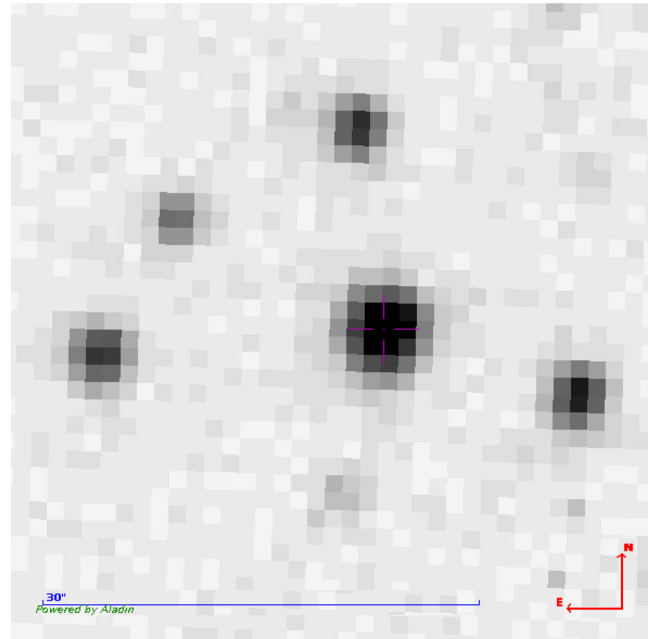
Figure 13. Image of transiting exoplanet candidate KPS-TF2-11789 as obtained with the MTM-500 telescope.
