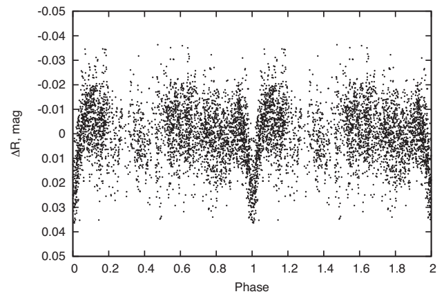
Figure 7. Phase-folded light curve of transiting exoplanet candidate KPS-TF1-19251 as obtained with the MASTER-II-Ural telescope.
