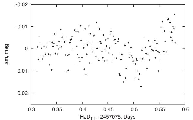
Figure 14. Secondary minimum of transiting exoplanet candidate KPS-TF2-11789 as obtained with the MTM-500 telescope. The theoretical time of the minimum (JD 2457075.51293) coincides with the minimum on the light curve.
