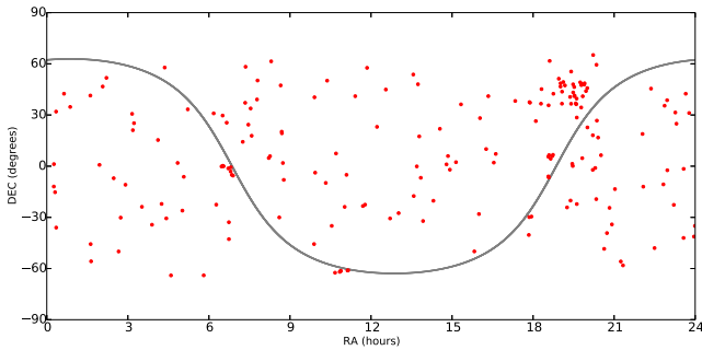
Figure 1. Spatial distribution of the known transiting hot Jupiters, i.e. exoplanets with orbital periods less than 10 d and with the minimum mass greater than 0.5M_J (Wright et al. 2011). The Galactic plane is shown by the grey solid curve.
