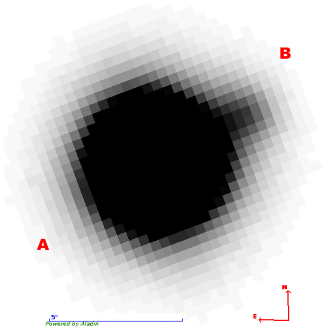
Figure 5. Image of transiting exoplanet candidate KPS-TF1-3154 as obtained with the SAO RAS 6-m telescope. The candidate represents a visual binary system.
