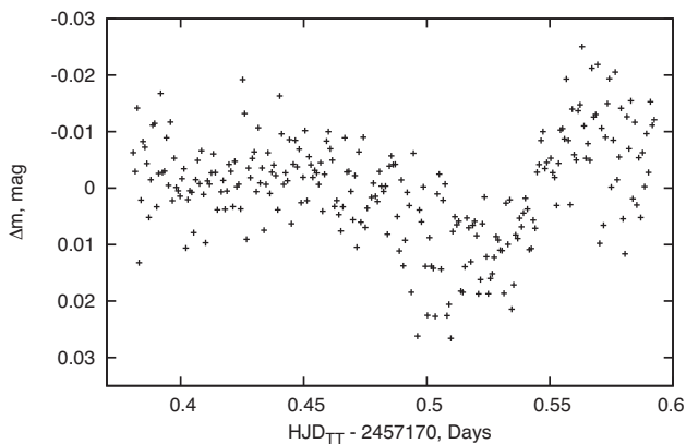
Figure 16. Single transit of the exoplanet candidate KPS-TF3-663 as obtained by the Baronnies Provençales Observatory telescope.
