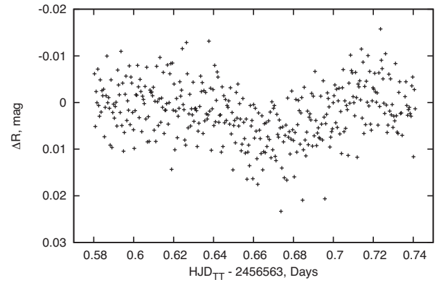
Figure 6. Secondary minimum of transiting exoplanet candidate KPS-TF1-3154 as obtained with the EdgeHD 11 SCT telescope (279 mm, f/7 ) installed at the Acton Sky Portal.
