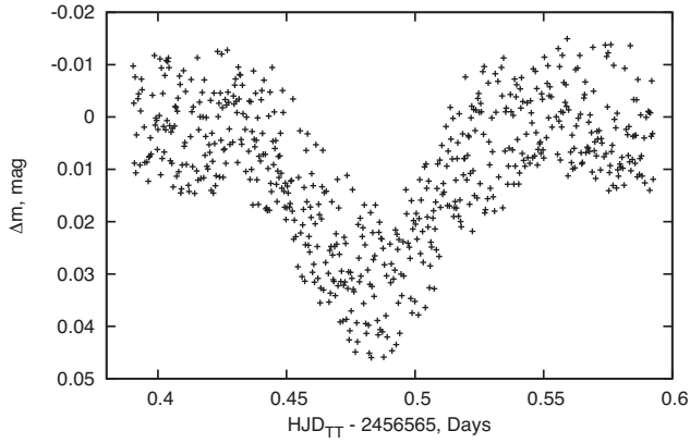
Figure 8. Single transit of the exoplanet candidate KPS-TF1-19251 as obtained with the 0.6-m Cassegrain telescope at the Centre for Astronomy of the Nicolaus Copernicus University in Torun (Poland).
