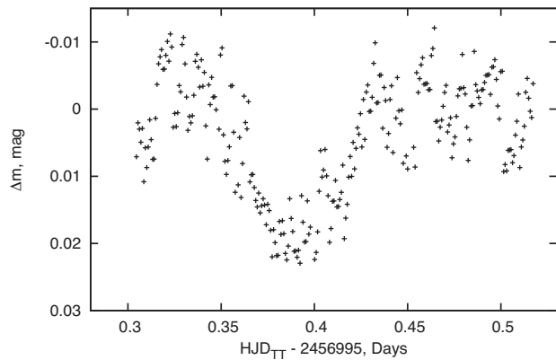
Figure 12. Single transit of the KPS-TF2-11789 exoplanet candidate as obtained with the MTM-500 telescope.
