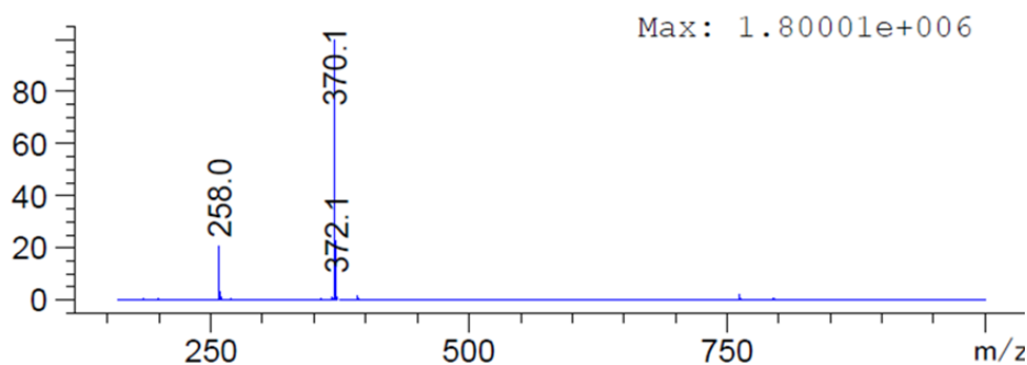
Figure 2. Mass fragmentation pattern of compound 8.8 (CID*, 200 eV)
