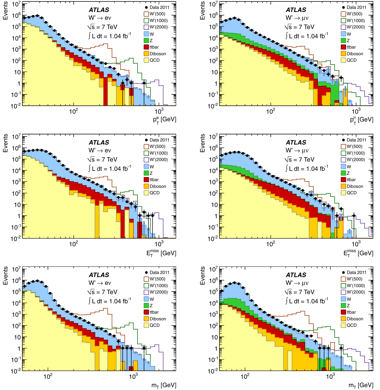
Fig. 1. Spectra of p_T (top), missing E_T (center) and m_T (bottom) for the electron (left) and muon (right) channels after event selection. The points represent data and the filled histograms show the stacked backgrounds. Open histograms are W' \rightarrow \ell \nu signals added to the background with masses in GeV indicated in parentheses in the legend. The QCD backgrounds estimated from data are also shown. The signal and other background samples are normalized using the integrated luminosity of the data and the NNLO (approximate-NNLO for t\bar{t} ) cross sections listed in Table 1.
